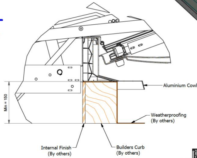
Detail C
